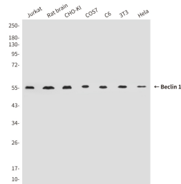
Western blot analysis of Beclin 1 in HeLa, 3T3, C6, COS7, CHO-K1, rat brain and Jurkat lysates using Beclin 1 antibody.
