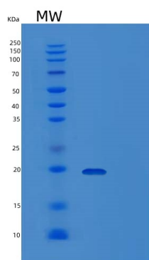
15% SDS PAGE(reduced) analysis of Recombinant Human KLRC3 Protein
