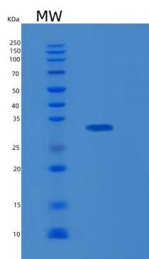
15% SDS PAGE(reduced) analysis of Recombinant Human LASP1 Protein
