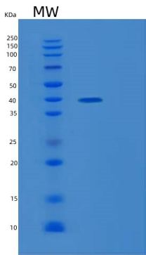
15% SDS PAGE(reduced) analysis of Recombinant Human MESDC1 Protein
