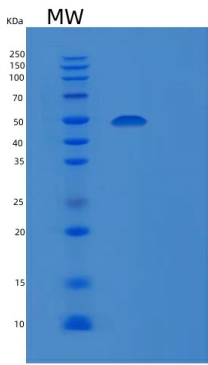
15% SDS PAGE(reduced) analysis of Recombinant Human PDHX Protein
