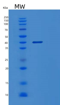
15% SDS PAGE(reduced) analysis of Recombinant Human POLB Protein
