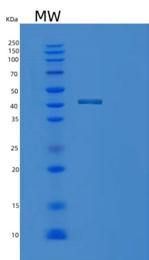
15% SDS PAGE(reduced) analysis of Recombinant Human PPME1 Protein
