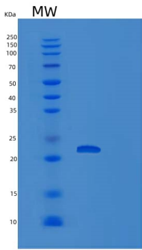
15% SDS PAGE(reduced) analysis of Recombinant Human REXO1 Protein
