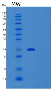
15% SDS PAGE(reduced) analysis of Recombinant Human SAR1B Protein
