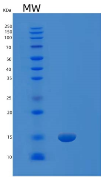
15% SDS PAGE(reduced) analysis of Recombinant Human SDHAF1 Protein
