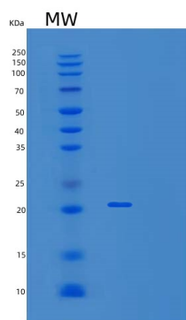
15% SDS PAGE(reduced) analysis of Recombinant Mouse SHH Protein
