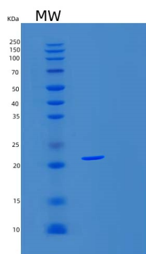
15% SDS PAGE(reduced) analysis of Recombinant Human SNAP25 Protein
