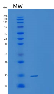
15% SDS PAGE(reduced) analysis of Recombinant Streptomyces Streptavidin Protein
