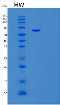
15% SDS PAGE(reduced) analysis of Recombinant Human UgDH Protein
