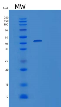
15% SDS PAGE(reduced) analysis of Recombinant Human 4-1BB/TNFRSF9/CD137 Protein(C-Fc)
