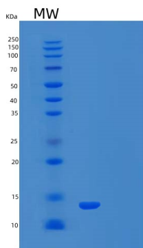
15% SDS PAGE(reduced) analysis of Recombinant Human S100 Calcium Binding Protein A9 Protein
