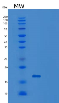
15% SDS PAGE(reduced) analysis of Recombinant Human BLyS / TNFSF13B / BAFF Protein
