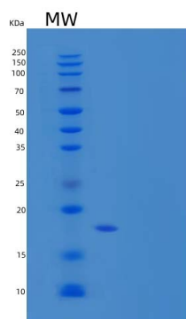
15% SDS PAGE(reduced) analysis of Recombinant Mouse CD83 Protein
