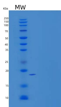
15% SDS PAGE(reduced) analysis of Recombinant Human Bcl-2-Like Protein 2/BCL2L2 Protein(C-6His)
