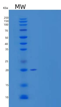
15% SDS PAGE(reduced) analysis of Recombinant Human Fibroblast Growth Factor 12/FGF-12 Protein
