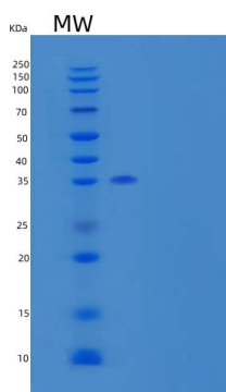
15% SDS PAGE(reduced) analysis of Recombinant Human Nectin-4/PVRL4 Protein(C-6His)
