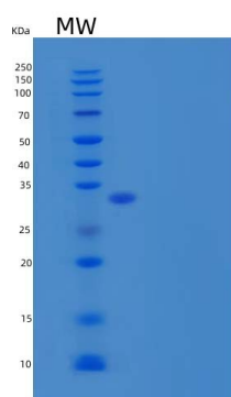
15% SDS PAGE(reduced) analysis of Recombinant Mouse Basigin Protein
