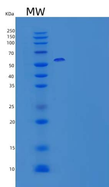
15% SDS PAGE(reduced) analysis of Recombinant Human Cytokine receptor common subunit gamma Protein
