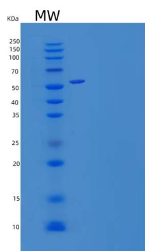
15% SDS PAGE(reduced) analysis of Recombinant Human Mothers Against Decapentaplegic Homolog 2/SMAD2 Protein(N-6His-Flag)
