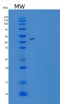
15% SDS PAGE(reduced) analysis of Recombinant Mouse T-lymphocyte surface antigen Ly-9 Protein
