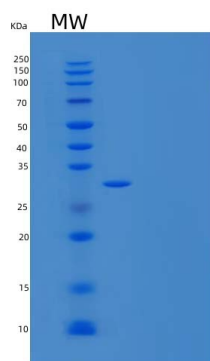
15% SDS PAGE(reduced) analysis of Recombinant Human NKG2A & CD94 Heterodimer Protein(N-8His & N-Flag)
