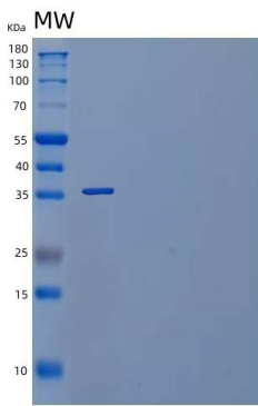
15% SDS PAGE(reduced) analysis of Recombinant Human C-X-C Motif Chemokine 10/CXCL10 Protein(C-Fc-6His)
