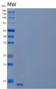
15% SDS PAGE(reduced) analysis of Recombinant Human C-X-C Motif Chemokine 5/CXCL5 Protein
