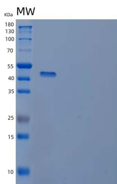
15% SDS PAGE(reduced) analysis of Recombinant Human Izumo sperm-egg fusion protein 4 Protein
