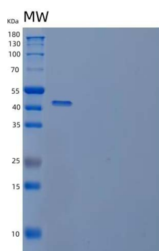
15% SDS PAGE(reduced) analysis of Recombinant Human Cystathionine \gamma -Lyase/CTH Protein
