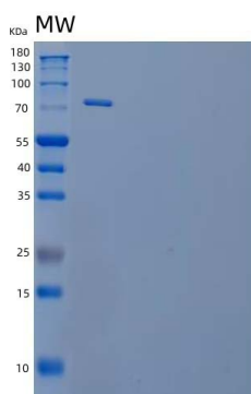
15% SDS PAGE(reduced) analysis of Recombinant Human Intercellular Adhesion Molecule 1/ICAM-1/CD54 Protein(C-Fc)
