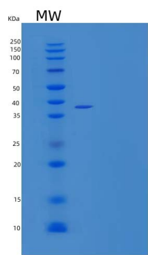
15% SDS PAGE(reduced) analysis of Recombinant Human Left-right Determination Factor 2 Protein(N-6His)
