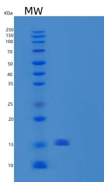
15% SDS PAGE(reduced) analysis of Recombinant Human Major Prion Protein/PRP/CD230 Protein
