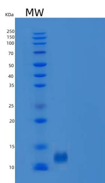
15% SDS PAGE(reduced) analysis of Recombinant Human B2M / Beta-2-microglobulin Protein (His tag)
