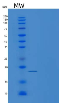
15% SDS PAGE(reduced) analysis of Recombinant Rat IL10 / Interleukin-10 Protein
