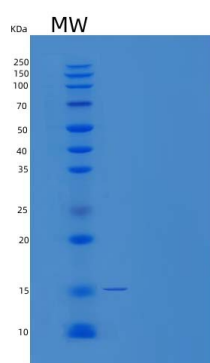
15% SDS PAGE(reduced) analysis of Recombinant Human Heat Shock Factor Protein 2/HSF2 Protein(N-6His)
