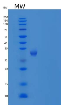
15% SDS PAGE(reduced) analysis of Recombinant Human Neurotrimin/NTRI Protein(C-6His)
