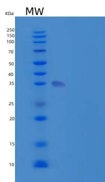
15% SDS PAGE(reduced) analysis of Recombinant Human IA2/PTPRN Protein(Met687-Gln979, N-6His)
