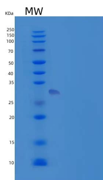
15% SDS PAGE(reduced) analysis of Recombinant Human IGF2 mRNA-Binding Protein 2/IGF2BP2/IMP2 Protein(C-6His, N-T7 tag)
