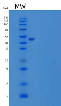
15% SDS PAGE(reduced) analysis of Recombinant Human TNF Receptor Superfamily Member 11B/OPG Protein(C-Fc)
