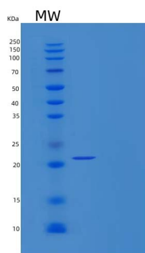
15% SDS PAGE(reduced) analysis of Recombinant Human PAPS Synthase 1/PAPSS1 Protein(C-6His)
