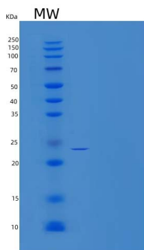
15% SDS PAGE(reduced) analysis of Recombinant Human Interleukin-12 Protein
