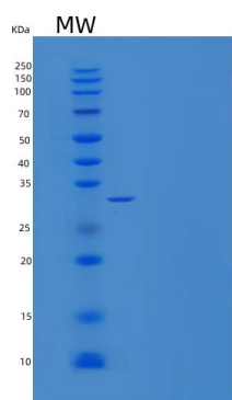
15% SDS PAGE(reduced) analysis of Recombinant Human C-X3-C Motif Chemokine 1/CX3CL1/Fractalkine Protein(C-6His)
