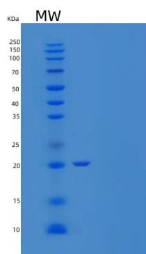
15% SDS PAGE(reduced) analysis of Recombinant Human Transcriptional Repressor Protein YY1 Protein(C-6His)
