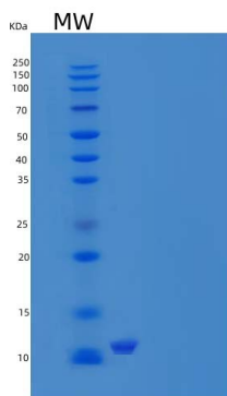
15% SDS PAGE(reduced) analysis of Recombinant Human Transforming Growth Factor \beta -3/TGFB3 Protein
