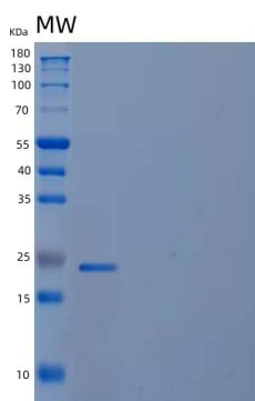
15% SDS PAGE(reduced) analysis of Recombinant Human Phosphomevalonate Kinase/PMVK Protein(N-6His)
