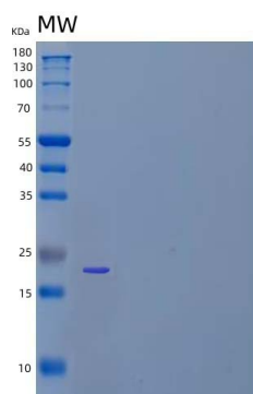
15% SDS PAGE(reduced) analysis of Recombinant Human LAIR-1/CD305 Protein(C-6His)
