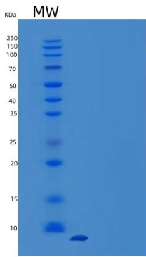
15% SDS PAGE(reduced) analysis of Recombinant Human C-C Motif Chemokine 2/CCL2/MCP-1 Protein
