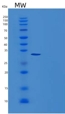
15% SDS PAGE(reduced) analysis of Recombinant Mouse Carbonic Anhydrase 4/CAN/CA4 Protein(C-6His)
