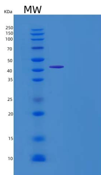
15% SDS PAGE(reduced) analysis of Recombinant Rat Cripto / TDGF1 Protein (Fc tag)
